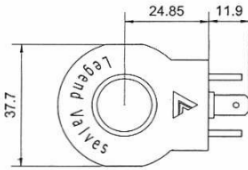
Model:LC-08-S-*H HIRSCHMANN
