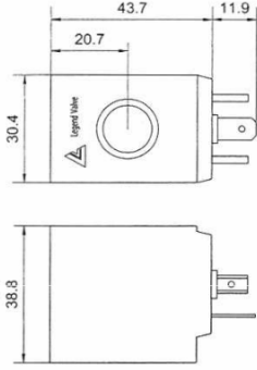
Model:LC-08-S-*H HIRSCHMANN
