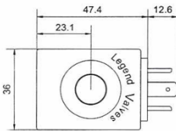
Model:LC3-10-C-*H HIRSCHMAN
