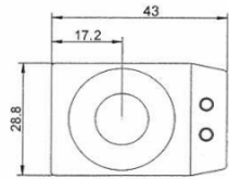
SINGLE LEAD
